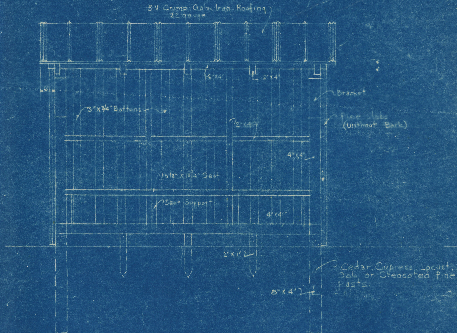
• FRONT ELEVATION • 1/2" = 12"
