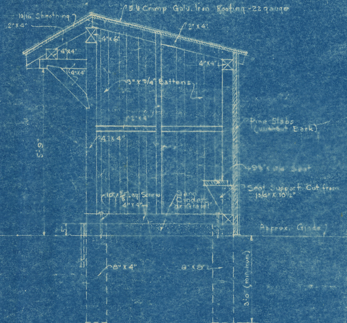
• SECTION • 1/2" = 12"
